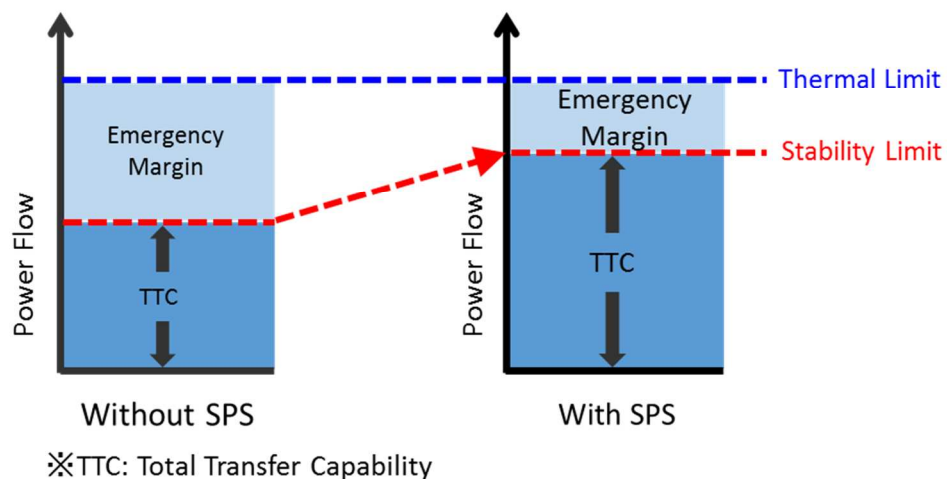
The Effective use of Emergency margin (capacity of the existing transmission lines reserved for accidental situations)
